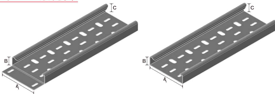
With built-in connector 連駁款
