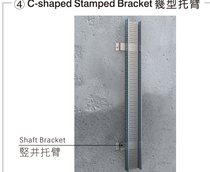
④ C-shaped Stamped Bracket 幾型托臂
