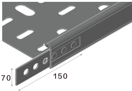
Tray side connector 托盤側連接
