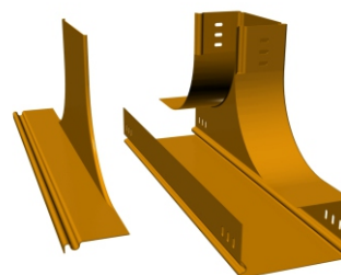
Vertical Tee with Down Outlet 下邊垂直三通 GY-QJ-C-2N
