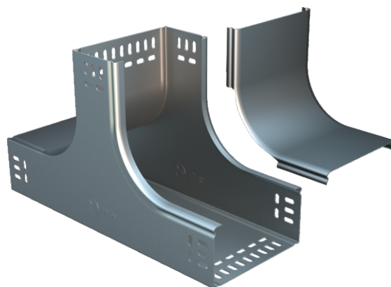
Vertical Tee-Downward Branch 下垂直三通 GY-QJ-P-2F
