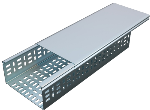
Straight Tray Section 直通 GY-QJ-P-1A
